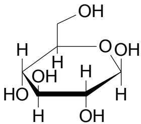
\beta -D-Glucopyranose
