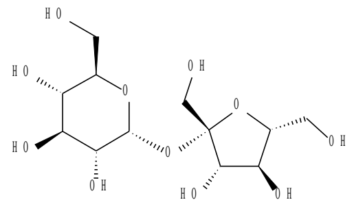
Sucrose [+JAN]-; [+USAN]-
