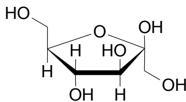
\beta -D-Fructofuranose
