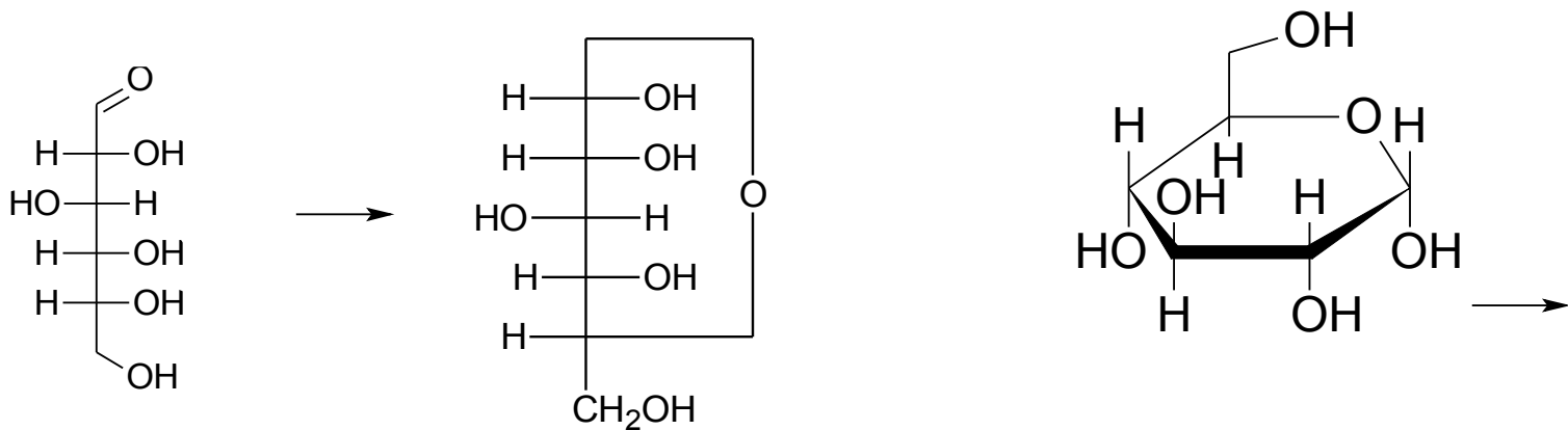
D-Glucose
